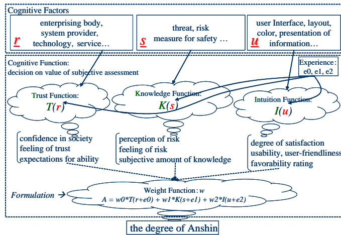
Figure.1: Anshin model
