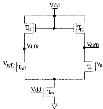
(a) Differential amplifier.
