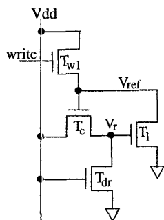
(a) V_{ref} generator.
