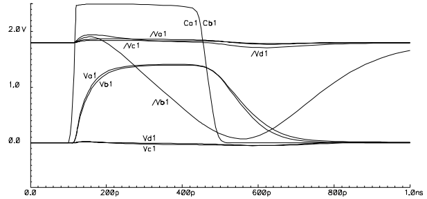
Fig. 6. Simulation of recovery from simultaneous SETs affecting enable lines C_a and C_b .
