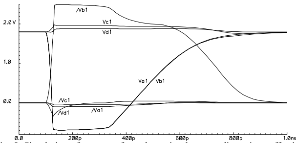
Fig. 5. Simulation of recovery from three simultaneous disruptions affecting V_a , V_b and /V_b .
