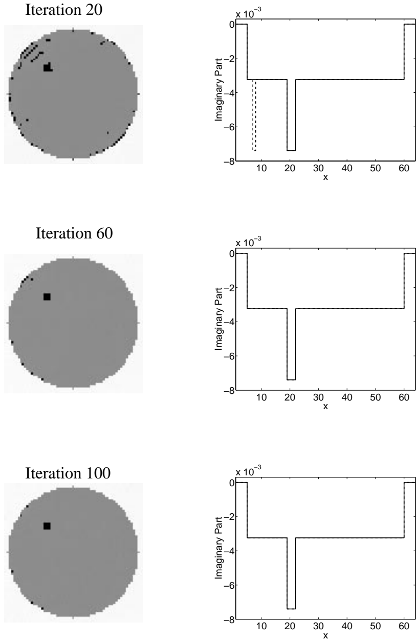
Fig. 14. Reconstructed results for the CGNN method for SNR = 50 dB (case 2). The left column shows the reconstructions at Iterations 20, 60 and 100. In the right column the solid lines are the true contrast along the line bisecting the tumor; the dashed lines are the reconstructed values for Iterations 20, 60 and 100.
