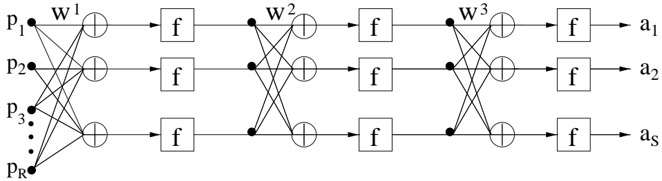
Fig. 2. Three-layer neural network.
