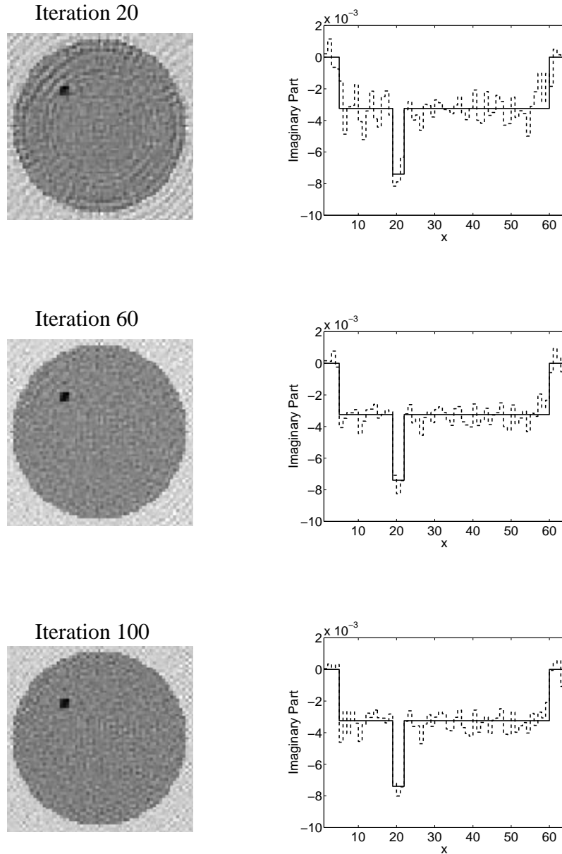
Fig. 15. Reconstructed results for the CG method for \text{SNR} = 50 dB (case 2). The left column shows the reconstructions at Iterations 20, 60 and 100. In the right column the solid lines are the true contrast along the line bisecting the tumor; the dashed lines are the reconstructed values for Iterations 20, 60 and 100.
