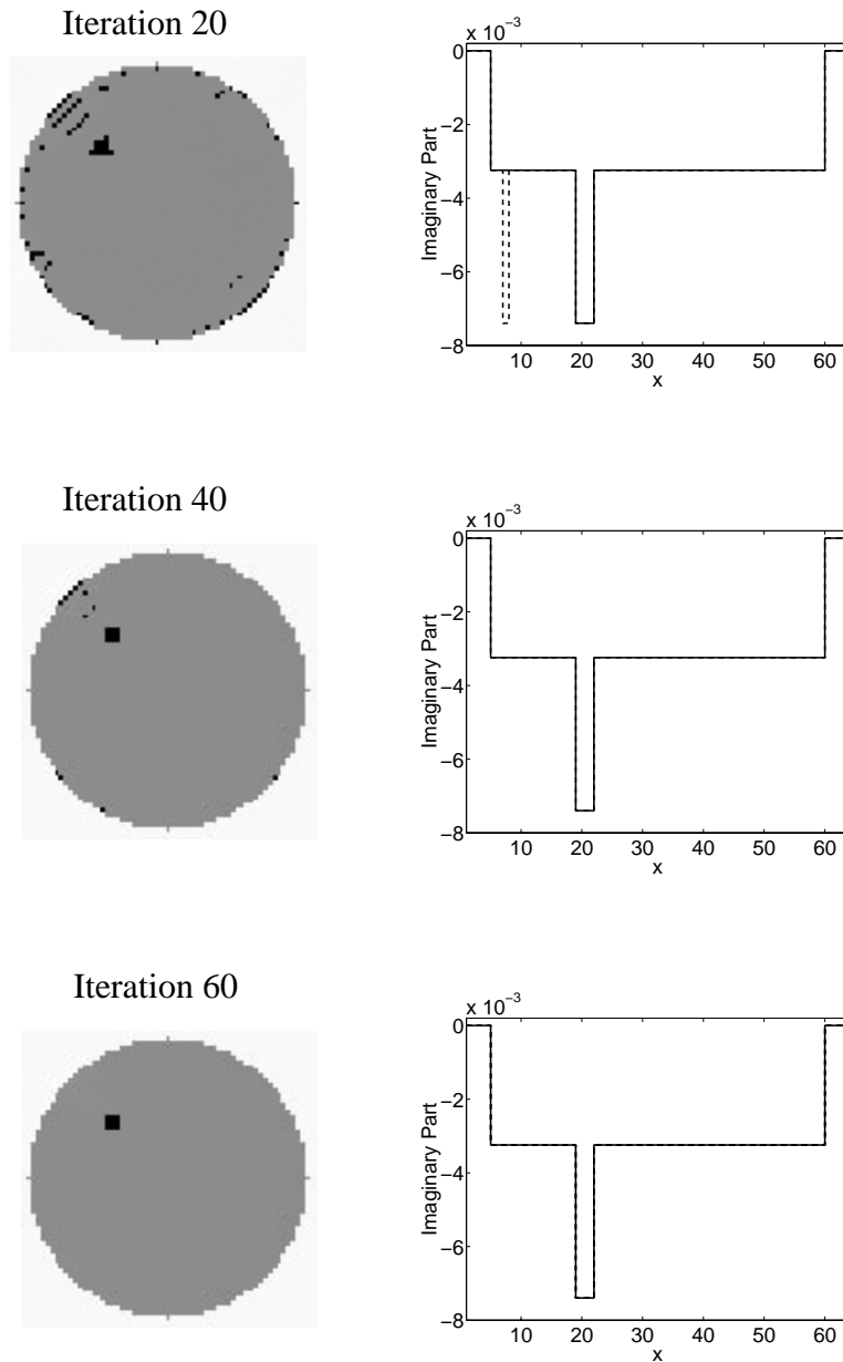
Fig. 11. Reconstructed results for the CGNN method for noiseless data (case 2). The left column shows the reconstructions at Iterations 20, 40 and 60. In the right column the solid lines are the true contrast along the line bisecting the tumor; the dashed lines are the reconstructed values for Iterations 20, 40 and 60.
