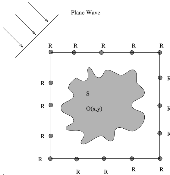
Fig. 1. Scattering geometry.
