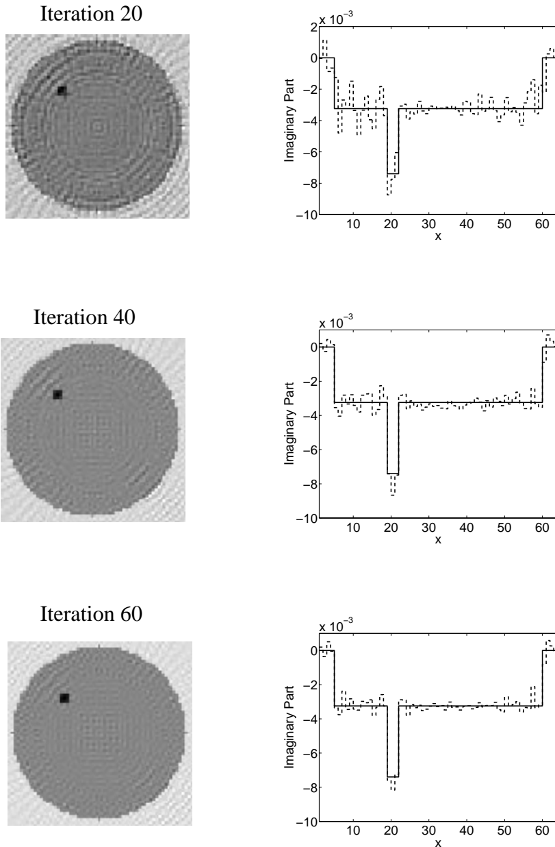
Fig. 12. Reconstructed results for the CG method for noiseless data (case 2). The left column shows the reconstructions at Iterations 20, 40 and 60. In the right column the solid lines are the true contrast along the line bisecting the tumor; the dashed lines are the reconstructed values for Iterations 20, 40 and 60.
