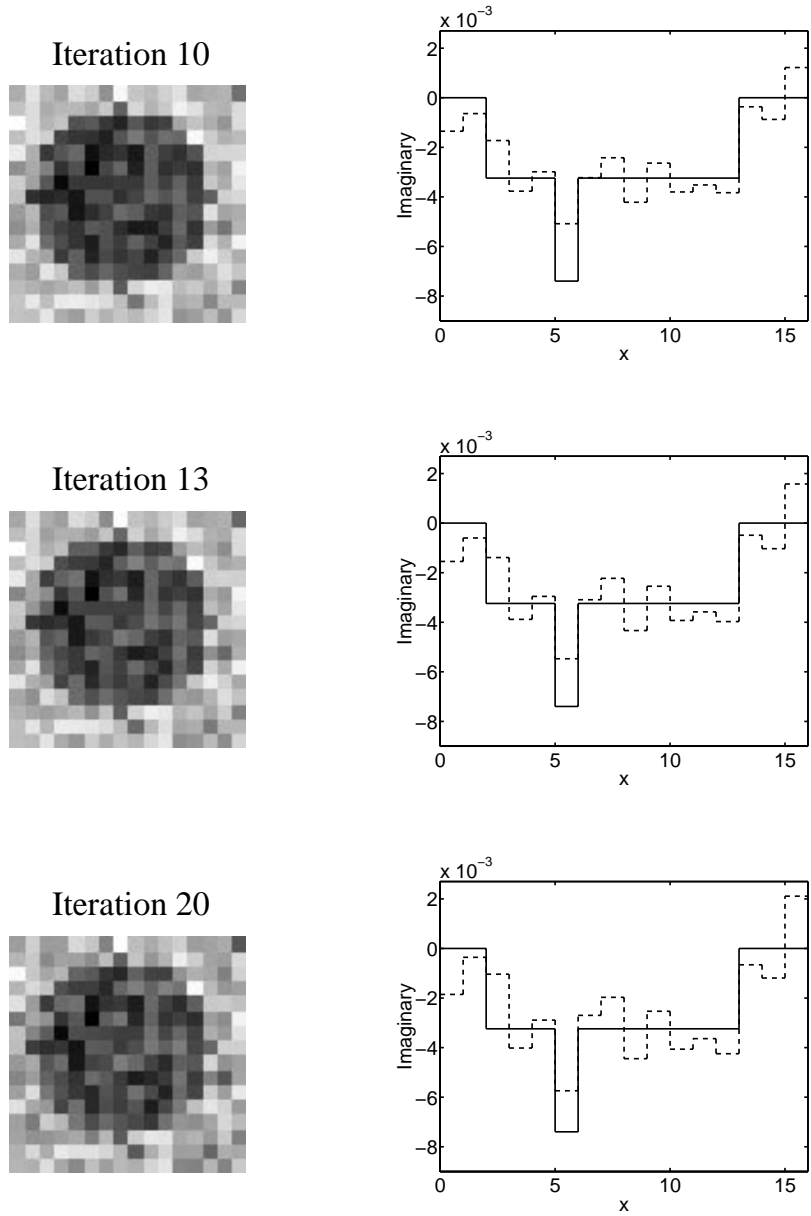
Fig. 10. Reconstructed results for the CG method for SNR = 35 dB (case 1). The left column shows the reconstructions at Iterations 10, 13 and 20. In the right column the solid lines are the true contrast along the line bisecting the tumor; the dashed lines are the reconstructed values for Iterations 10, 13 and 20.
