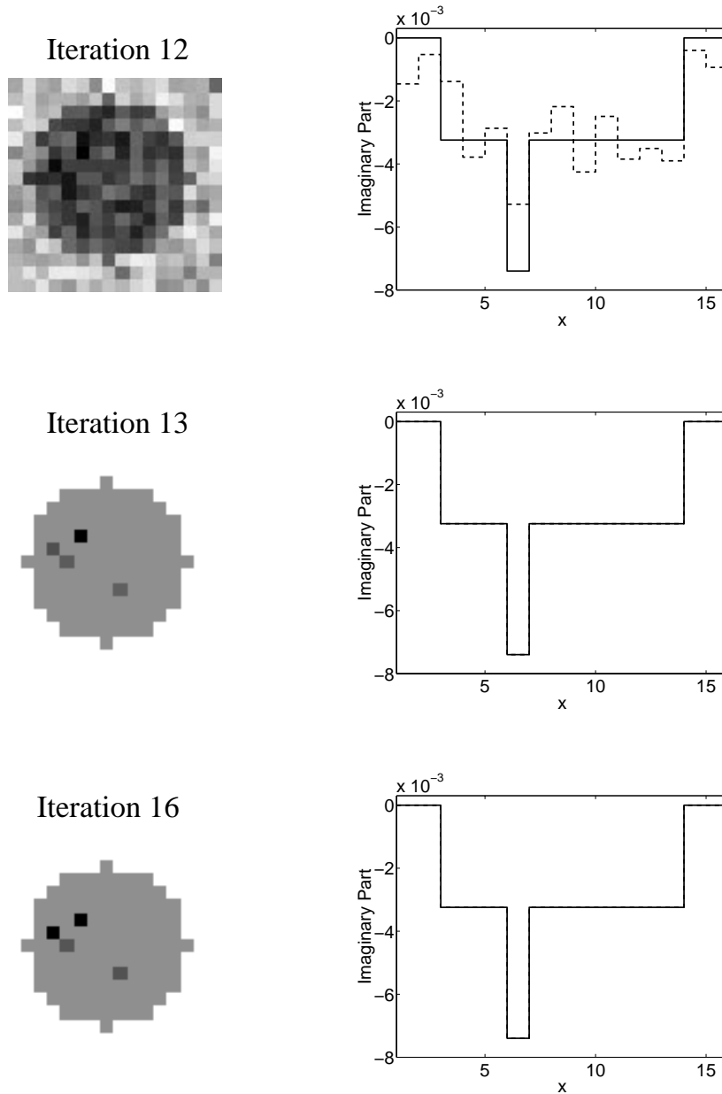
Fig. 9. Reconstructed results for the CGNN method for SNR = 35 dB (case 1). The left column shows the reconstructions at Iterations 12, 13 and 16. In the right column the solid lines are the true contrast along the line bisecting the tumor; the dashed lines are the reconstructed values for Iterations 12, 13 and 16.
