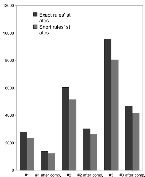
Fig. 1. Number of NFA states
