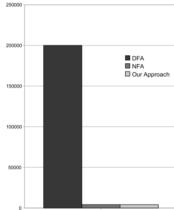
Fig. 6. Memory consumption
