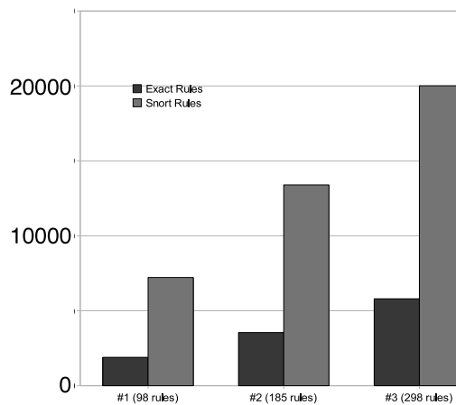
Fig. 2. Number of NFA transitions
